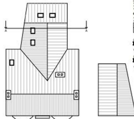
Proposed Roof Plan - 1:100
