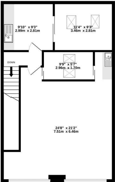
FIRST FLOOR 793 sq.ft. (73.7 sq.m.) approx.
