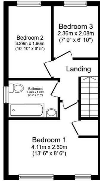
First Floor Floor area 31.7 sq.m. (342 sq.ft.)
