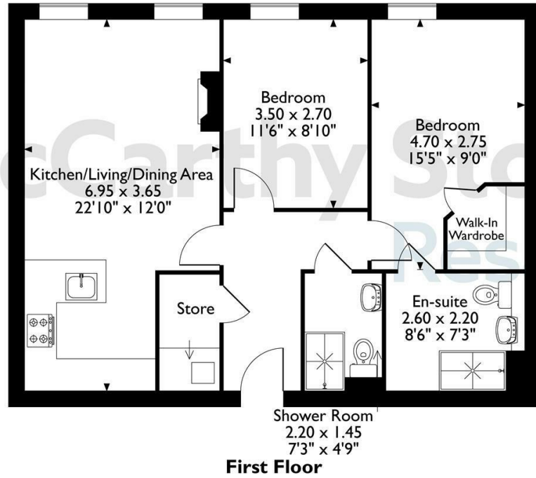
The position & size of doors, windows, appliances and other features are approximate only. © ehouse. Unauthorised reproduction prohibited. Drawing ref. dig/8667026/DST.
