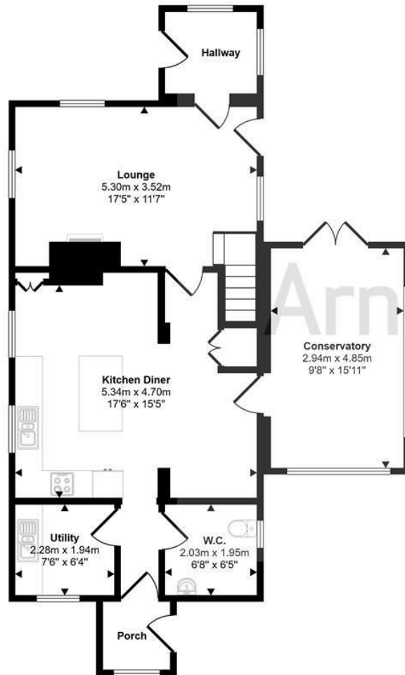
Ground Floor Approx 80 sq m / 863 sq ft
