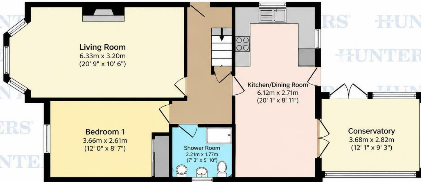
GROUND FLOOR
