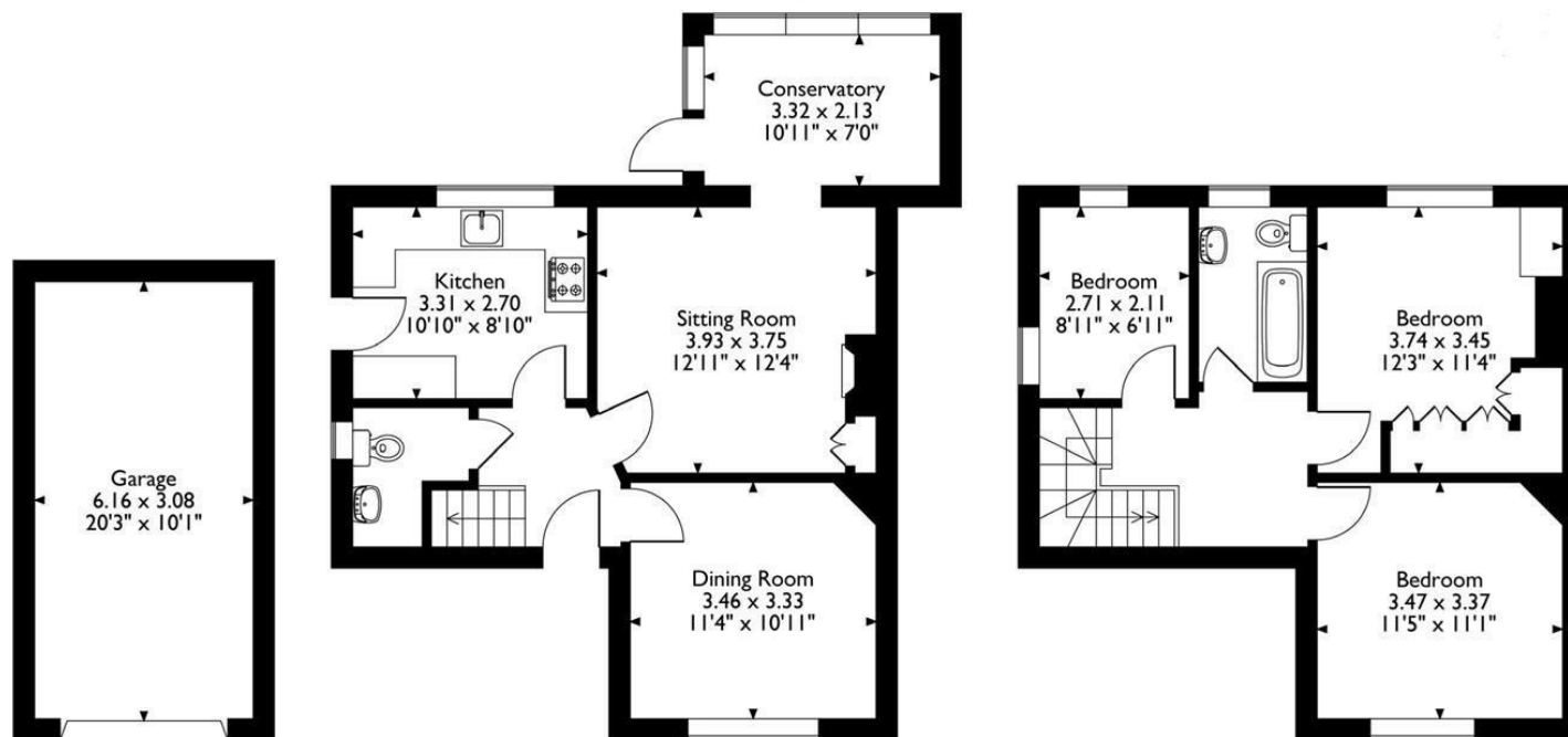
Ground Floor
