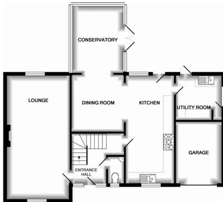
GROUND FLOOR APPROX. FLOOR AREA 944 SQ.FT. (87.7 SQ.M.)
