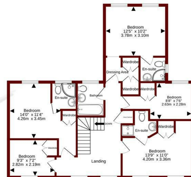
1st Floor 872 sq.ft. (81.0 sq.m.) approx.
