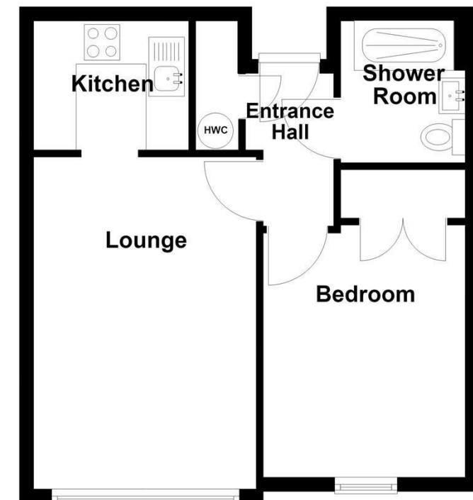
Total area: approx. 38.3 sq. metres (412.6 sq. feet) 44 Champions Court, Henlow Drive, Dursley, GL11 4BE
