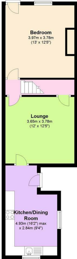
Ground Floor Approx. 45.1 sq. metres (485.9 sq. feet)
