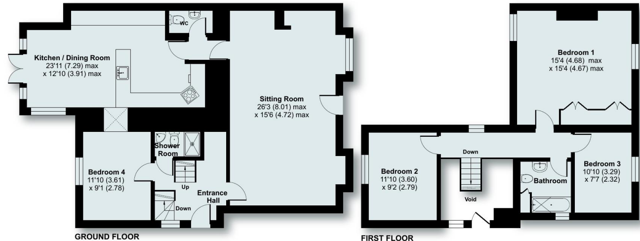
GROUND FLOOR
