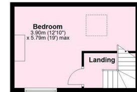
Second Floor Approx. 22.9 sq. metres (248.4 sq. feet)
