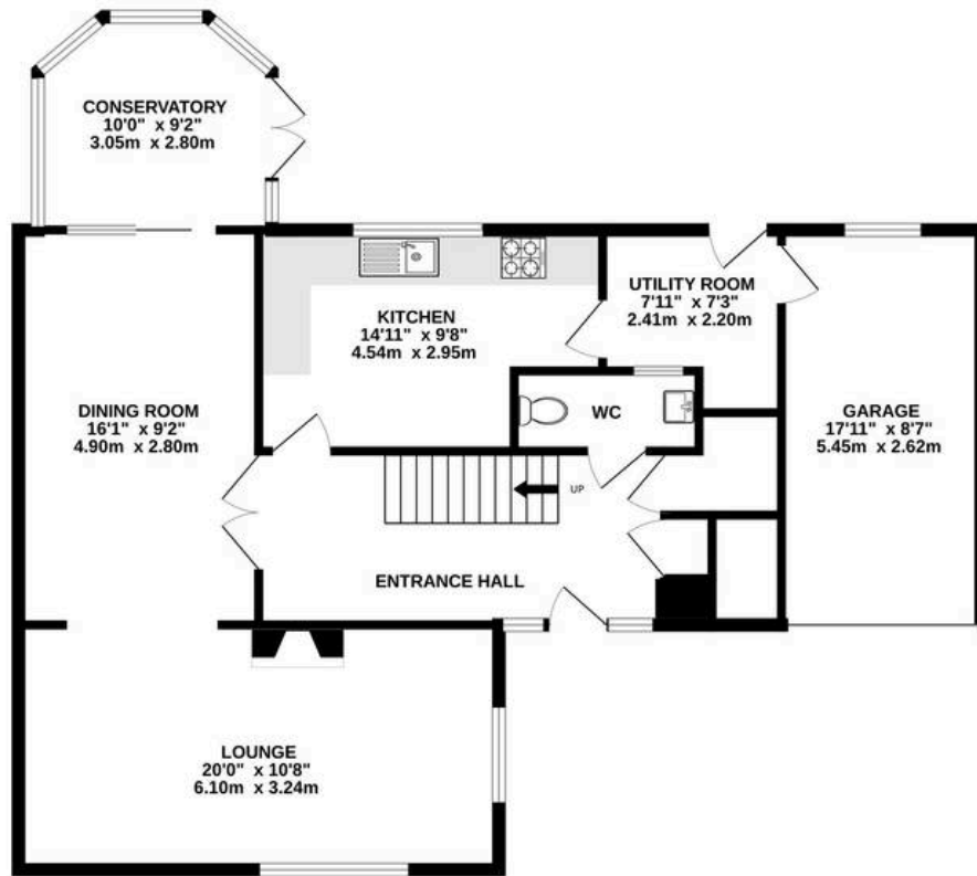
GROUND FLOOR 1012 sq.ft. (94.0 sq.m.) approx.
