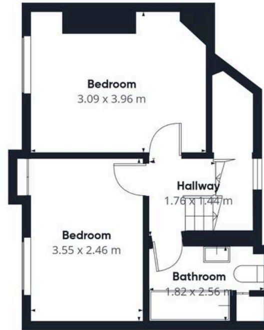
Floor 1
