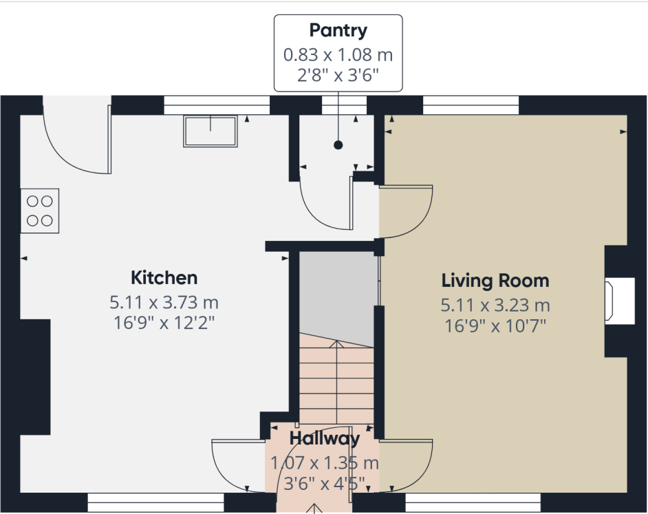
Floor 0 Building 1
