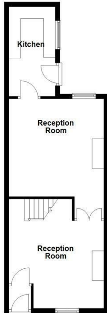
Ground Floor Approx. 43.4 sq. metres (467.1 sq. feet)
