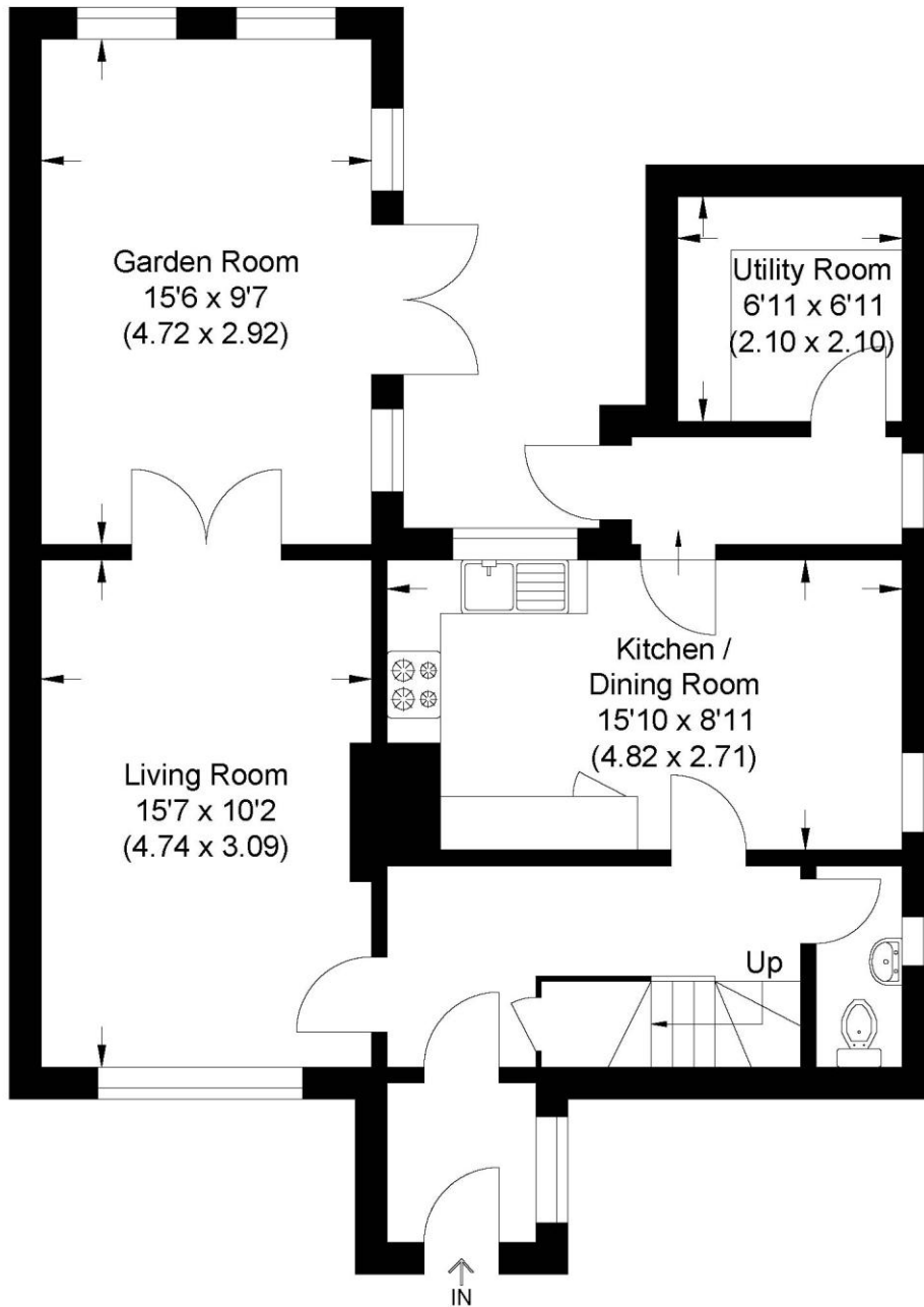
Ground Floor
