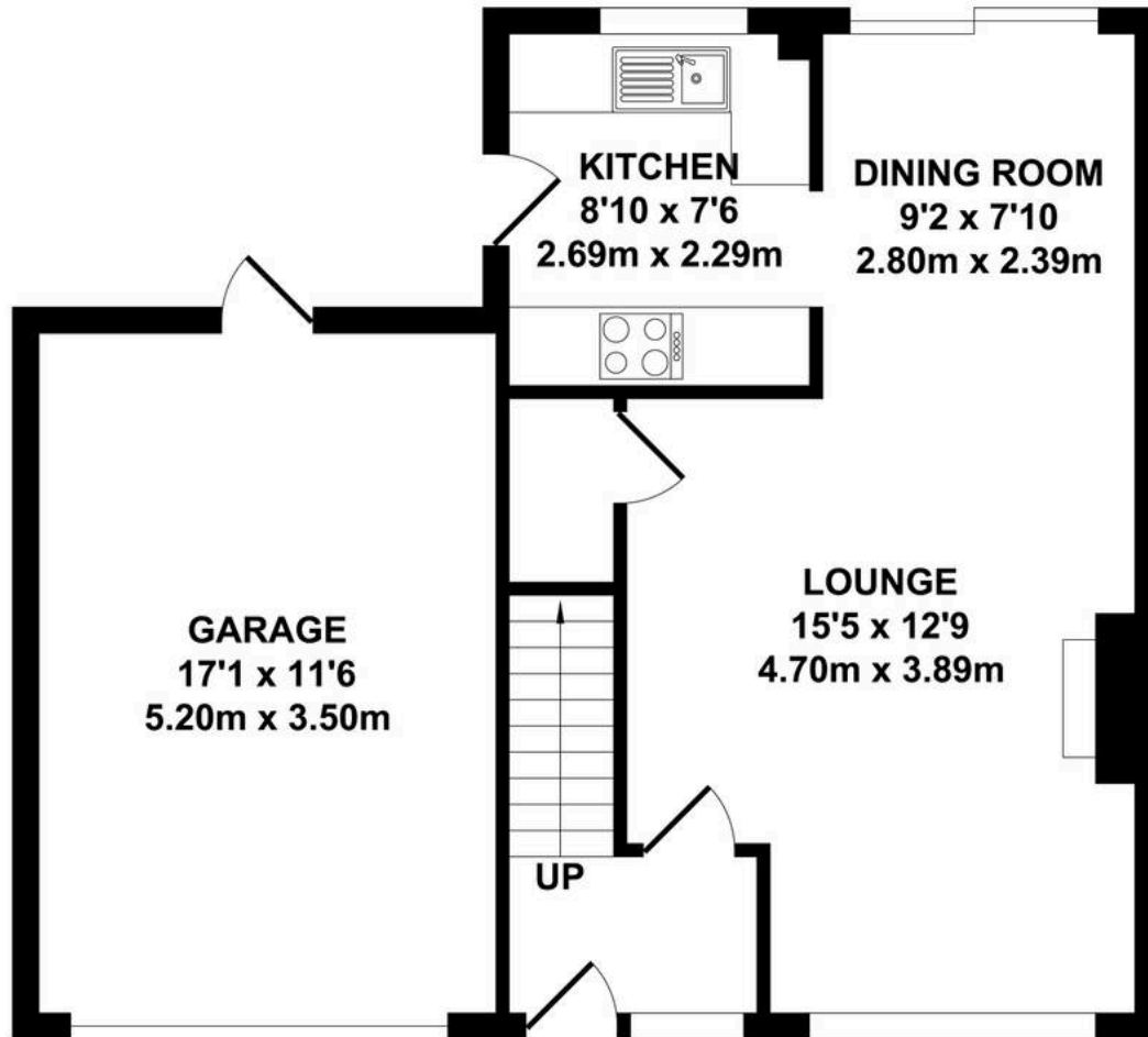
GROUND FLOOR APPROX. FLOOR AREA 587 SQ.FT. (54.60 SQ.M.)
