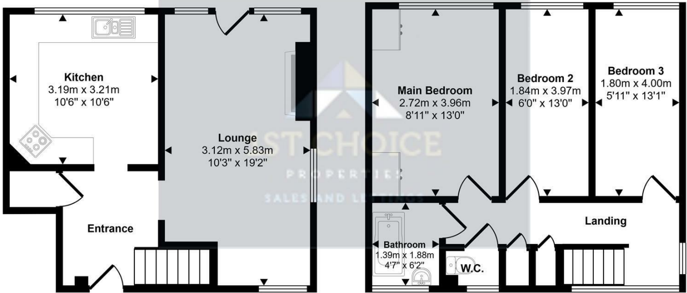
Ground Floor Approx 36 sq m / 388 sq ft
