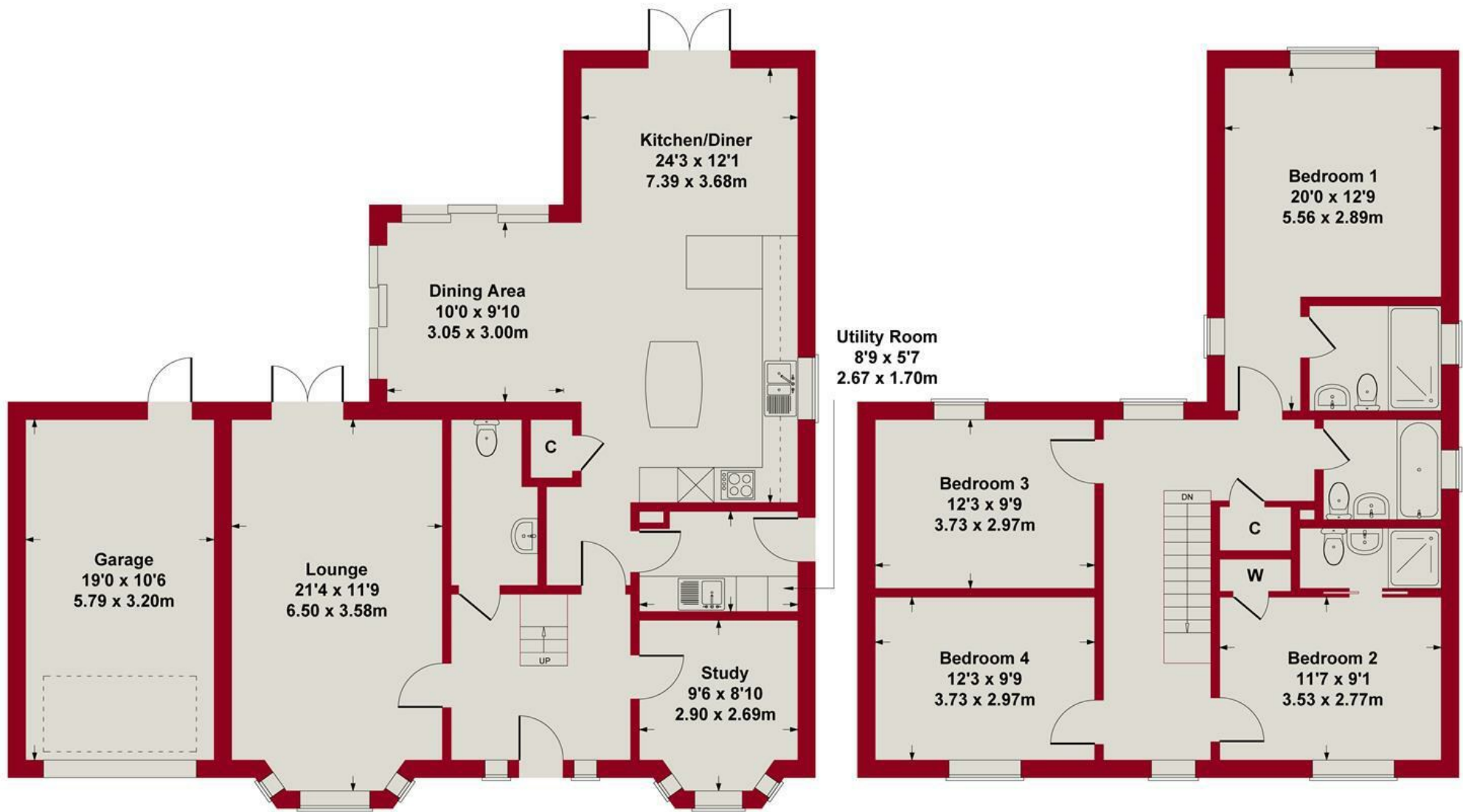
FIRST FLOOR
