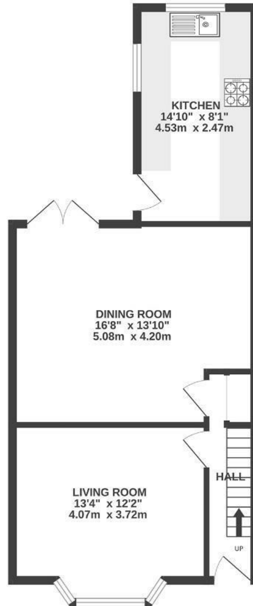
GROUND FLOOR
