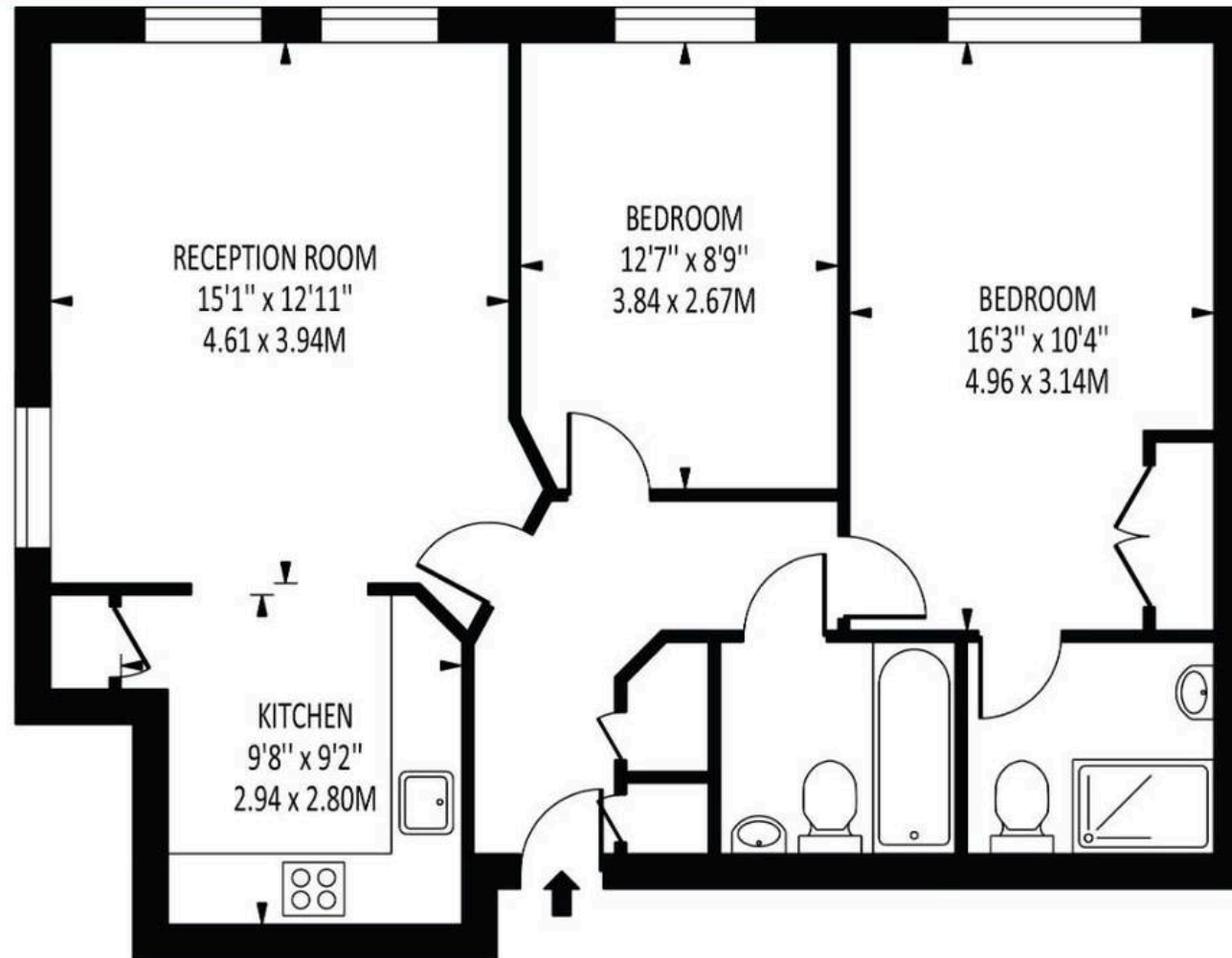
GROUND FLOOR
