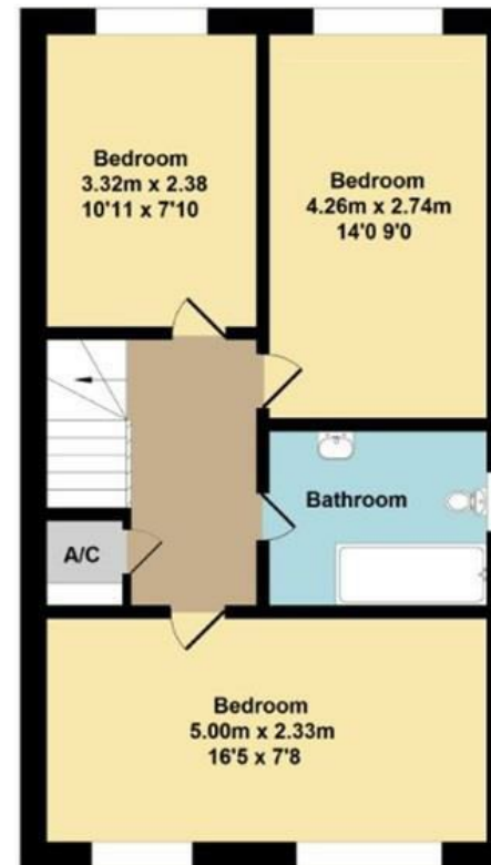
First Floor Approx. Floor Area 46.00 Sq.M. (496 Sq.Ft.)
