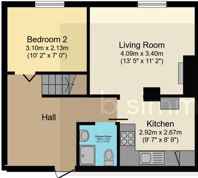
First Floor Floor area 44.9 sq.m. (484 sq.ft.)
