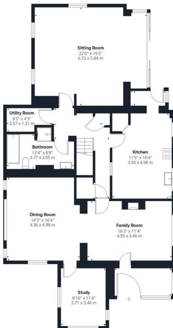
Ground Floor Building 1
