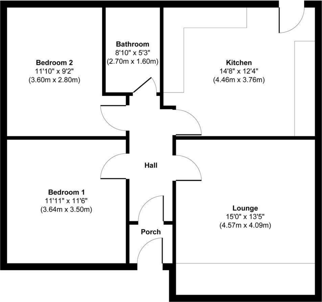
Floor Plan
