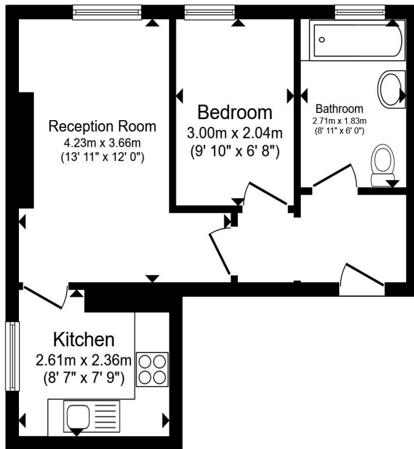
Floor Plan
