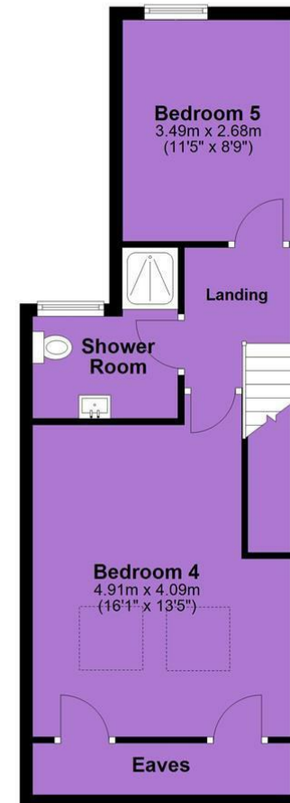
Second Floor
