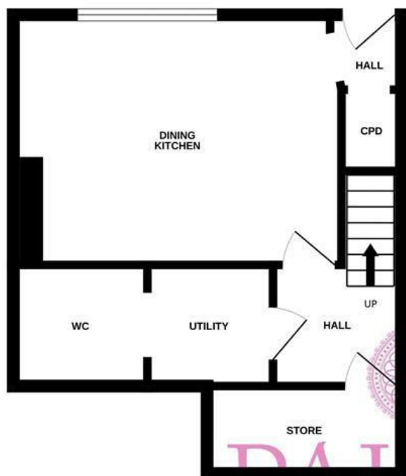
BASEMENT LEVEL
