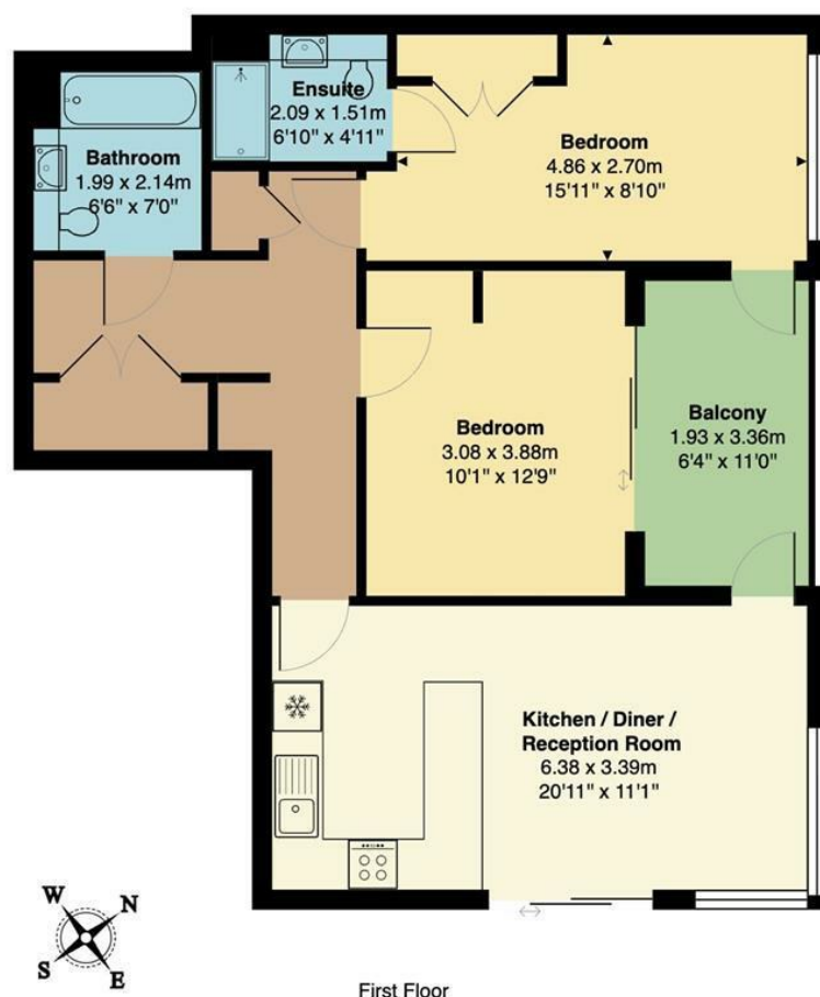
First Floor Total Area: 69.3 m 2 ... 746 ft 2 (excluding balcony) All measurements are approximate and for display purposes only
