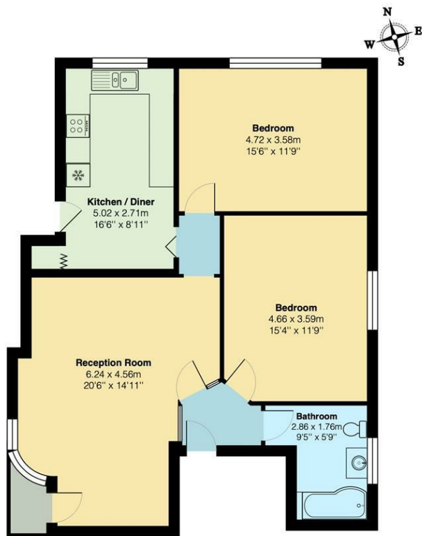
Second Floor
