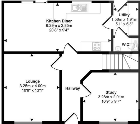
Ground Floor Approx 56 sq m / 601 sq ft
