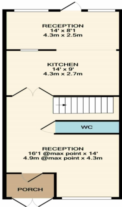
GROUND FLOOR APPROX. FLOOR AREA 671 SQ.FT. (62.3 SQ.M.)
