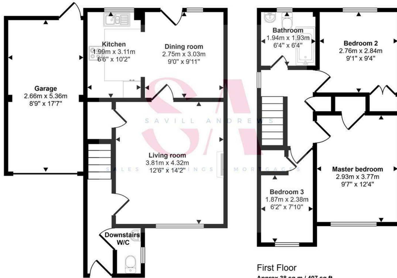
Ground Floor Approx 55 sq m / 589 sq ft
