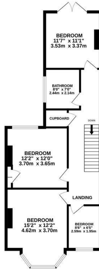
1ST FLOOR
