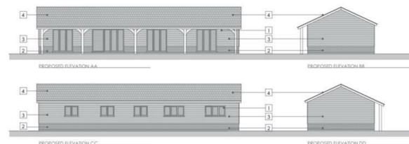
PROPOSED ELEVATIONS
