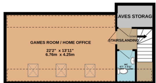
GARAGE BLOCK 1ST FLOOR 428 sq.ft. (39.8 sq.m.) approx.
