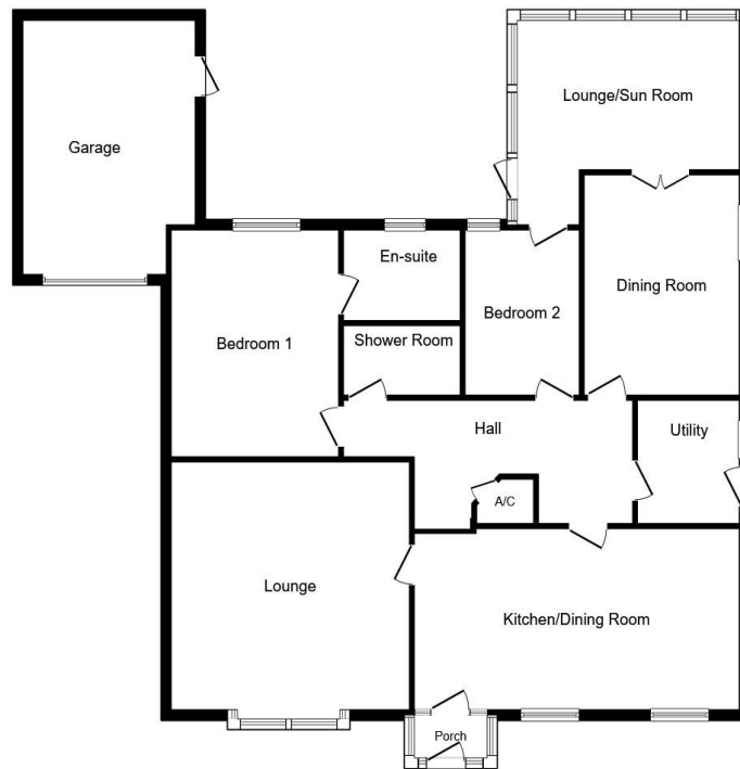
floor plan 1
