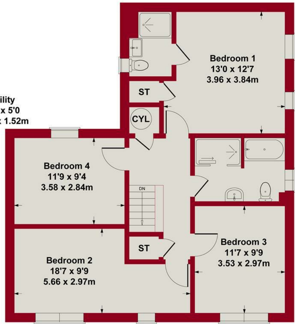
FIRST FLOOR
