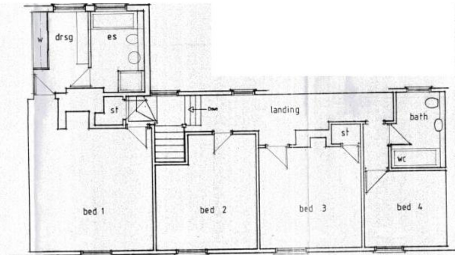
Proposed First Floor Plan Scale 1:50
