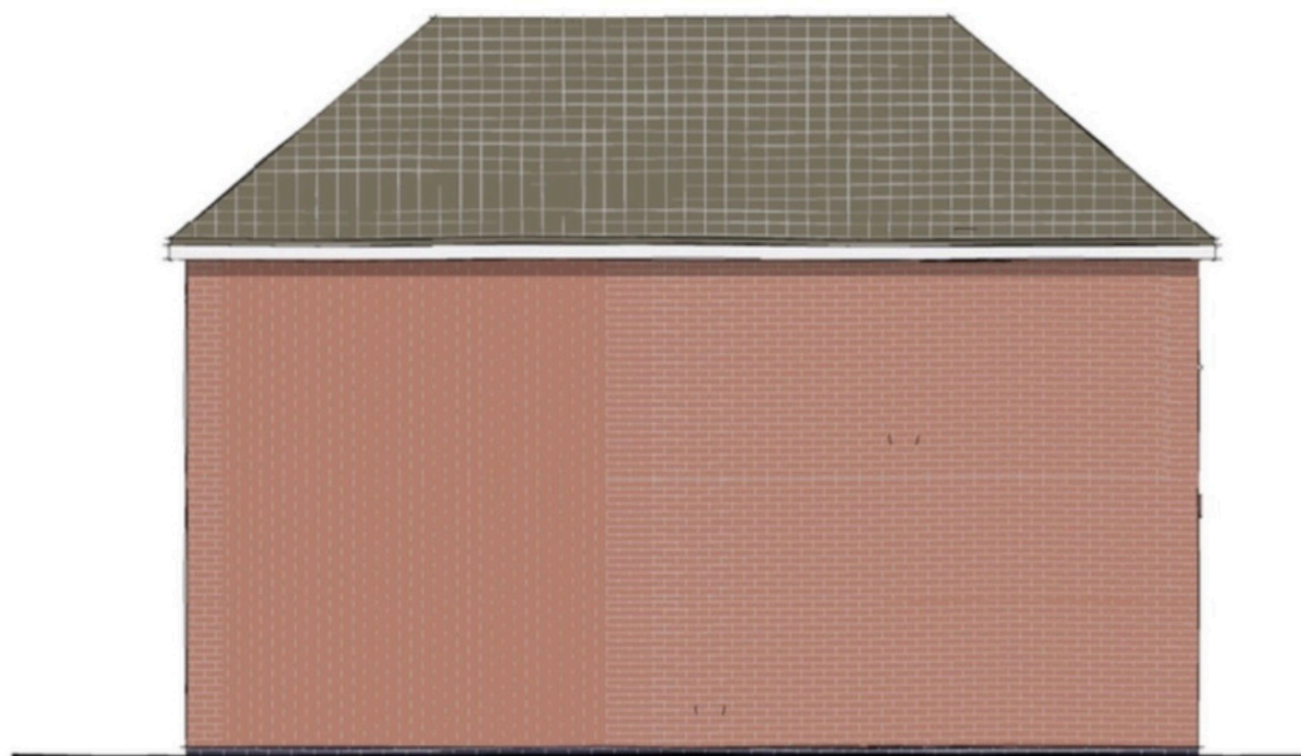
East Elevation 1:50
