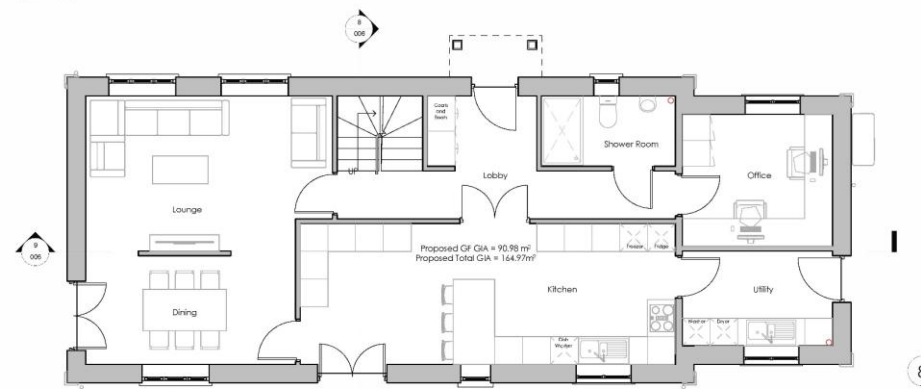
1 Plot 2 - Proposed Ground Floor Plan 1:50
