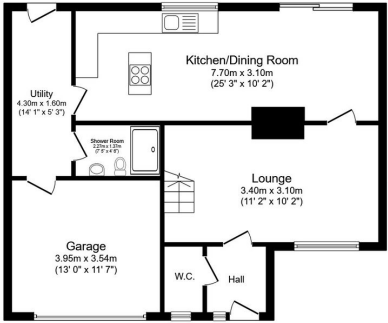
Ground Floor Floor area 73.4 sq.m. (790 sq.ft.)
