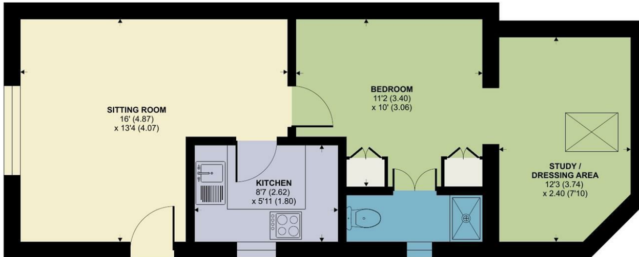
GROUND FLOOR
