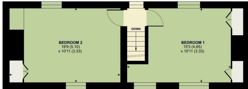
FIRST FLOOR
