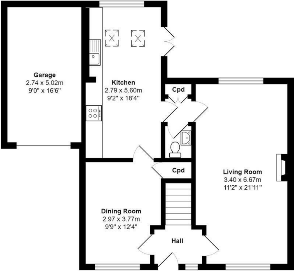
Ground Floor
