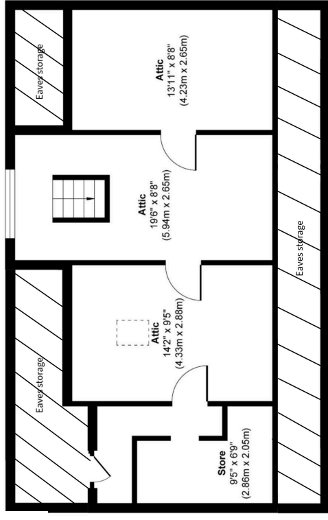
Second Floor Approximate Floor Area 496 sq. ft. (46.12 sq. m)
