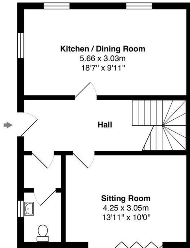
Ground Floor Area: 47.2 m 2 ... 508 ft 2
