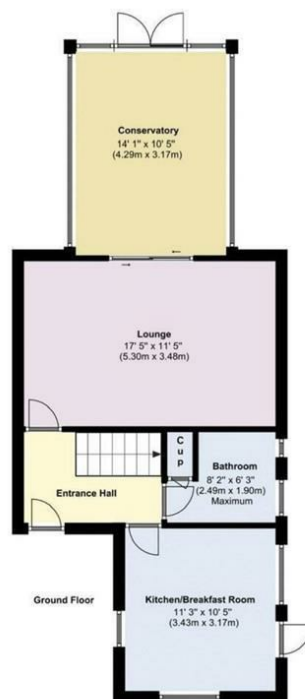
Floor plan 2
